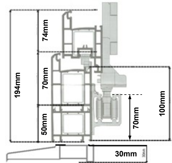
6. Low Threshold Open OUT [Internal Doors ONLY]
