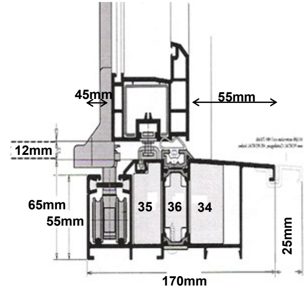
6. Low Threshold Open OUT [Internal Doors ONLY]
