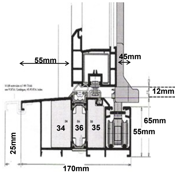
5. Low Threshold Open IN
