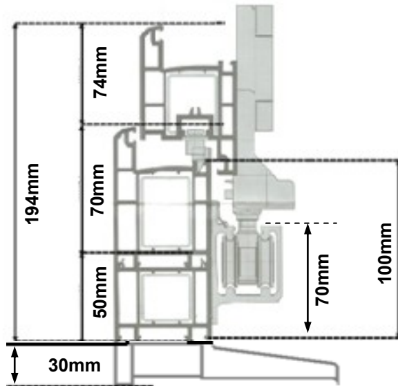
4. BOTTOM Running Open OUT
