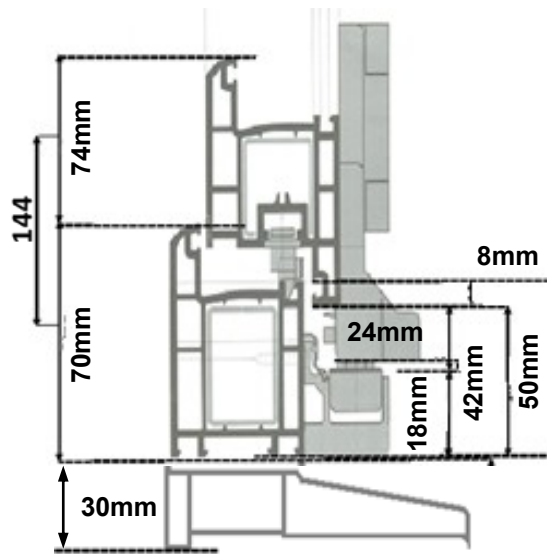
2. TOP Running Open OUT
